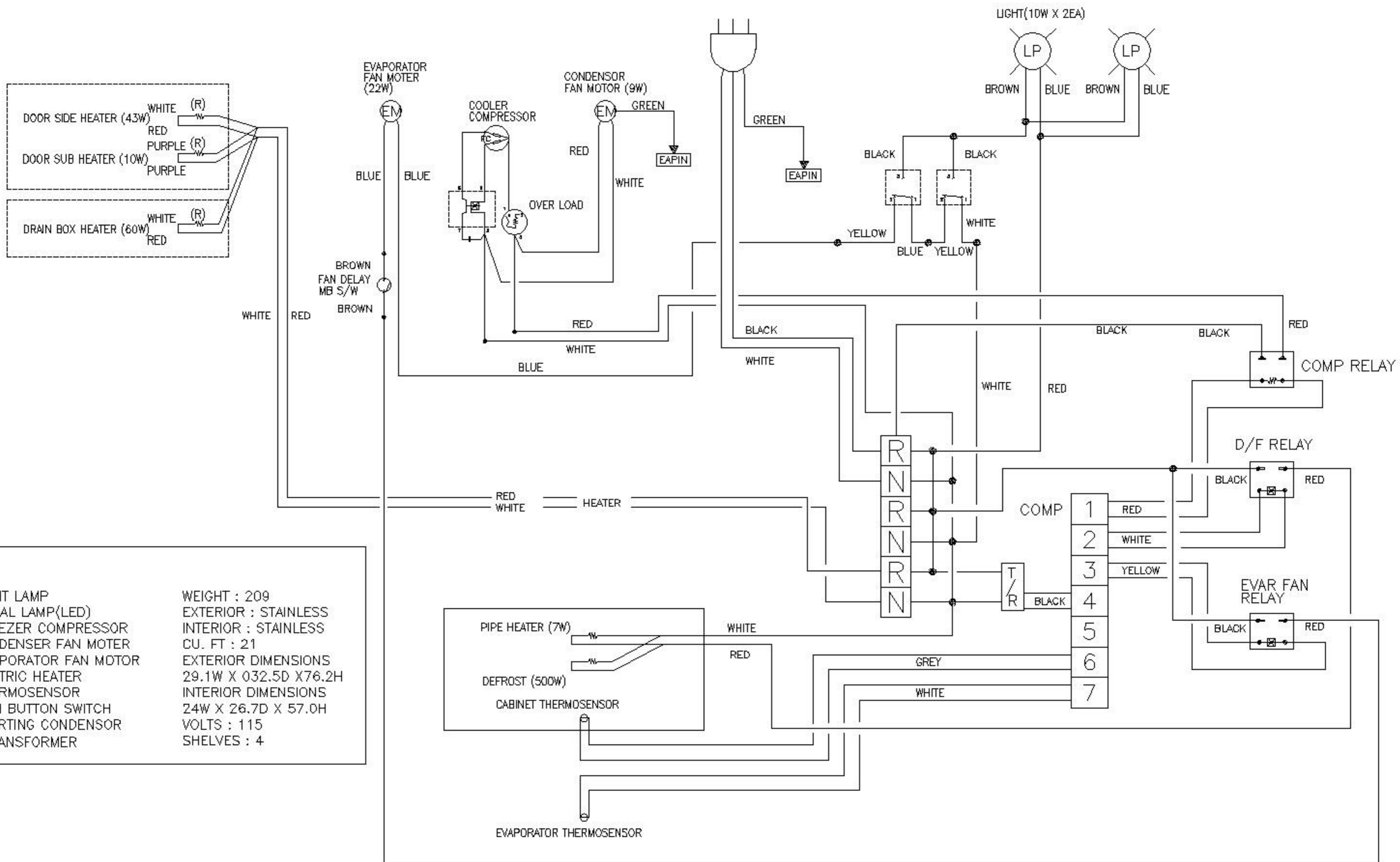
CONTROL WIRING DIAGRAM(U2CFF-16C) AC 115V X 60Hz X 1Ph
